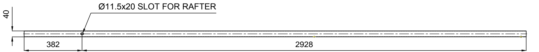
BOTTOM VIEW
