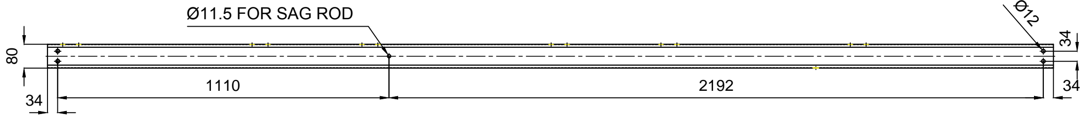
FRONT VIEW
