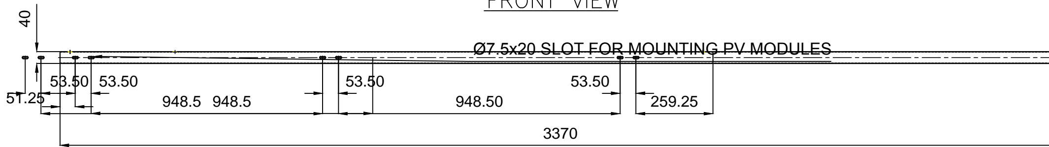
FRONT VIEW
