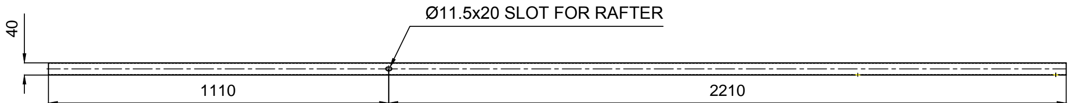
BOTTOM VIEW
