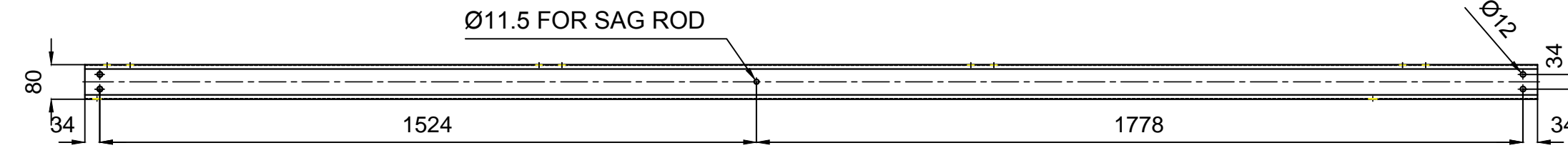
FRONT VIEW
