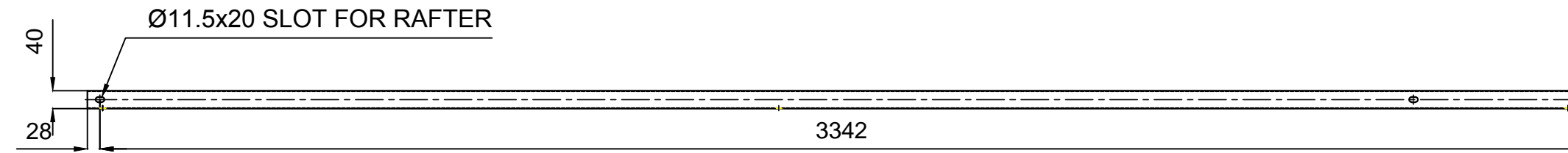
BOTTOM VIEW
