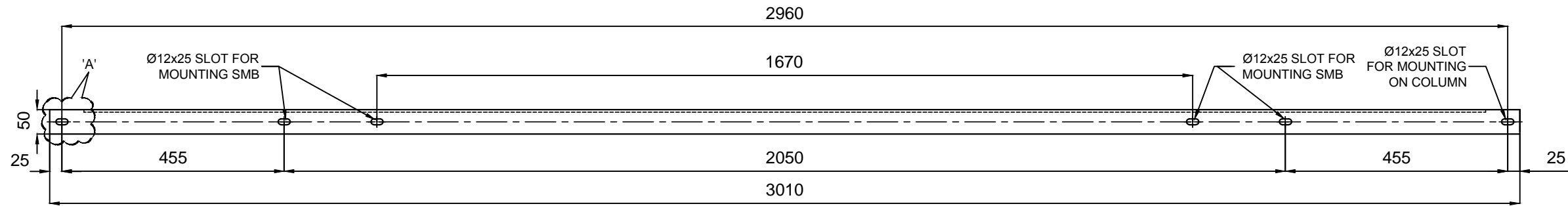
FRONT VIEW
