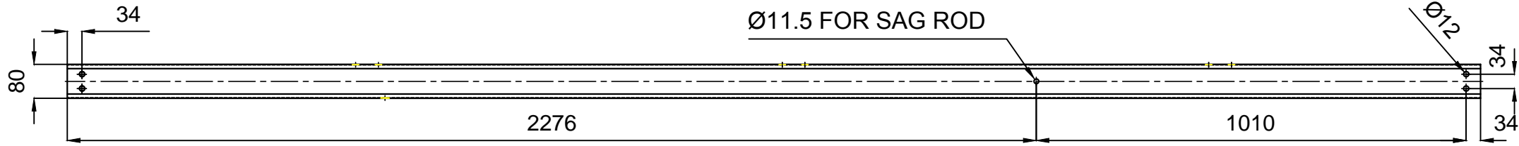
FRONT VIEW
